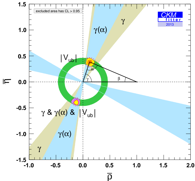
FIG. 3: The allowed region in the \rho - \eta plane, assuming that tree diagrams are dominated by the Standard Model [12].
