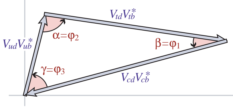
FIG. 6: Graphical representation of the unitarity constraint V_{ud}V_{ub}^* + V_{cd}V_{cb}^* + V_{td}V_{tb}^* = 0 as a triangle in the complex plane.
