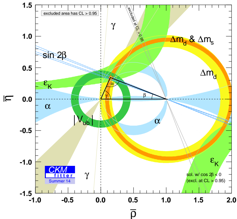
FIG. 2: Allowed region in the \rho, \eta plane. Superimposed are the individual constraints from charmless semileptonic B decays ( |V_{ub}/V_{cb}| ), mass differences in the B^0 ( \Delta m_d ) and B_s ( \Delta m_s ) neutral meson systems, and CP violation in K \rightarrow \pi\pi ( \varepsilon_K ), B \rightarrow \psi K ( \sin 2\beta ), B \rightarrow \pi\pi, \rho\pi, \rho\rho ( \alpha ), and B \rightarrow DK ( \gamma ). Taken from [12].
