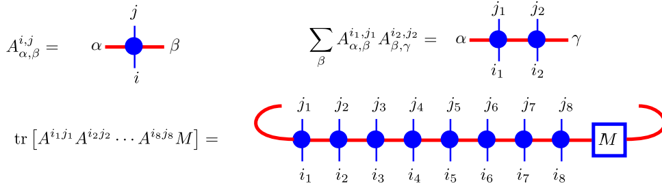
Figure 1: Graphical notation of a tensor contraction and of a matrix product operator.
