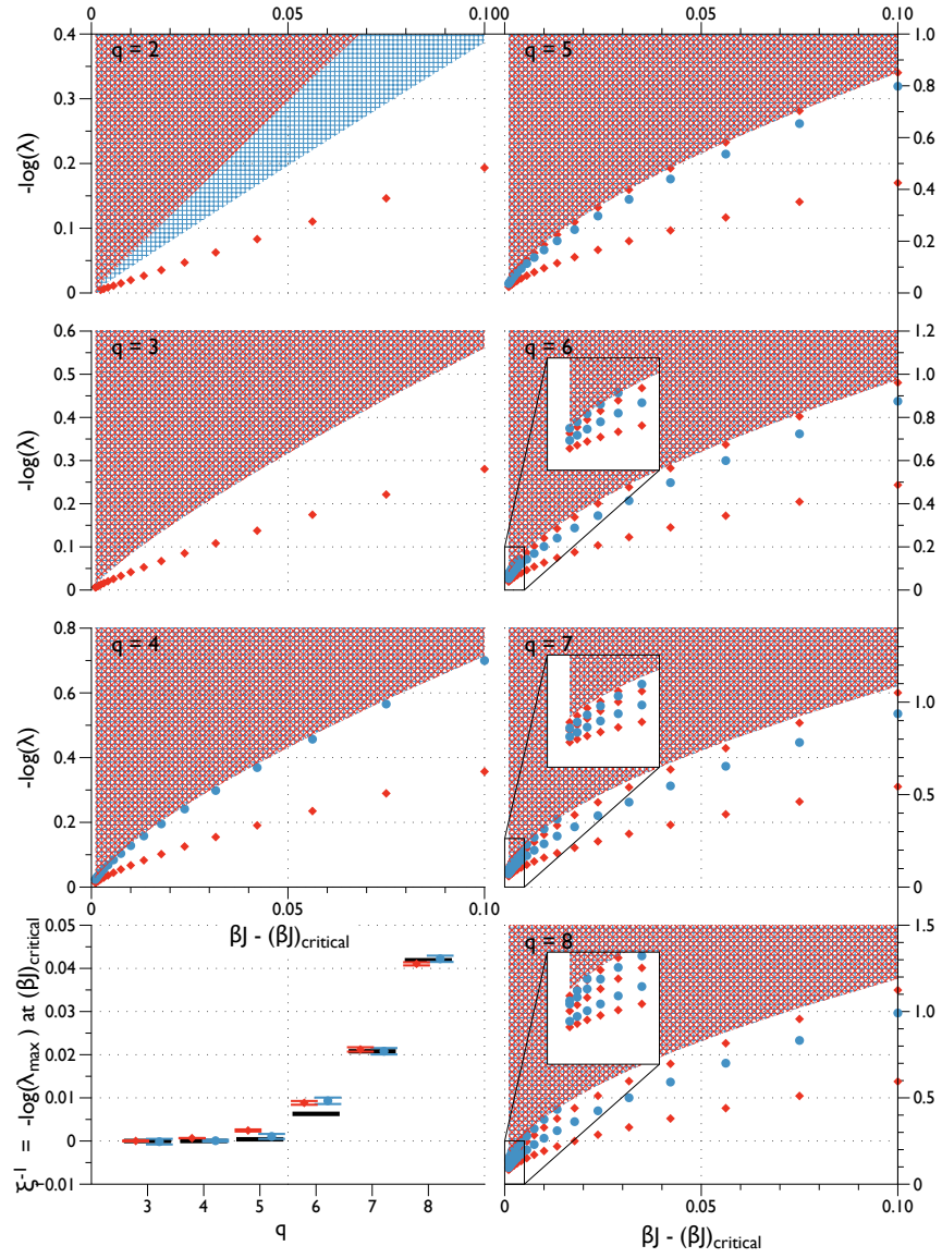
Figure 24: Transfer matrix spectra at zero momentum of the q -level Potts model for q = 2, 3, \dots, 8 in the ordered (symmetry-broken) phase \beta J > (\beta J)_c = \log(\sqrt{q} + 1) , plotted as function of \beta J . Blue dots indicate topologically trivial excitations, whereas red diamonds are obtained with the topologically non-trivial ansatz. Blue arced region (horizontal and vertical) indicate continuous bands in the trivial sector, whereas red diagonally arced regions indicate bands in the topological sector. Lower left panel shows the extrapolated largest eigenvalue at (\beta J)_c , with the exact values in black. See text for additional discussion.
