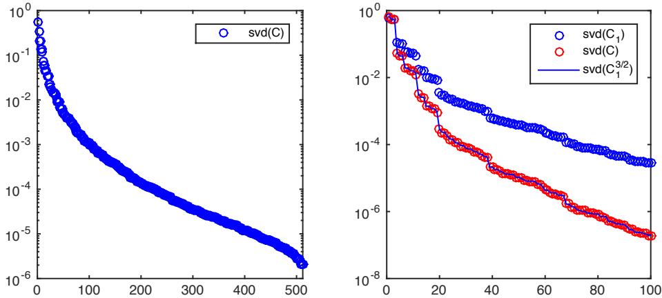
Figure 26: Left (a): Schmidt spectrum of the MPS approximation with D = 512 to the ground state of the Heisenberg model, or equivalently, the fixed point of the transfer matrix of the 6-vertex model. Right (b): Schmidt spectrum of the fixed point of the PEPS transfer matrix of the filtered Fibonacci string net model, as well as spectrum of the CTM. These two spectra are equal up to a power 3/2 , related to the geometric interpretation where C represents a corner of 180^\circ and C_1 represents a corner of 120^\circ .
