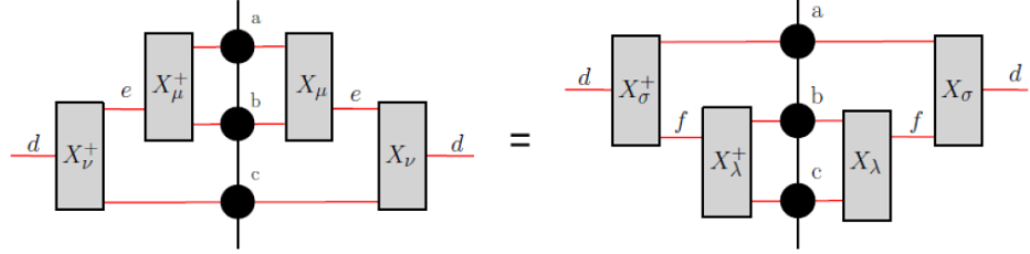
Figure 16: Associativity conditions for the fusion tensors X .
