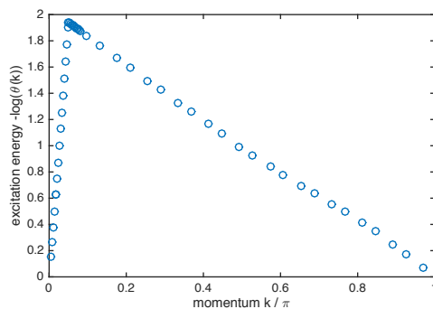
Figure 27: Energy momentum spectrum of the entanglement Hamiltonian of the chiral spin liquid PEPS of Ref. [134], computed directly in the thermodynamic limit using the MPS methods presented in this section.
