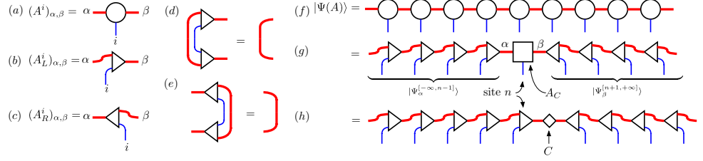
Figure 20: The matrix product state (MPS) tensor (a) and its left (b) and right (c) normal forms as defined by the isometric constraints shown in panels (d) and (e). This allows expressing the uniform MPS (f) in the form (g) or (h) corresponding to Eq. (3) or Eq. (2), respectively.
