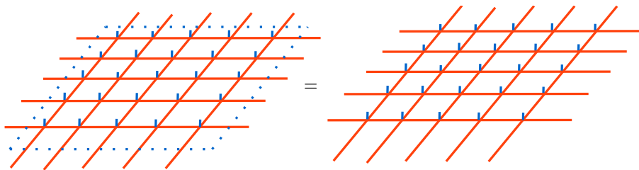
Figure 7: For a topologically ordered projected entangled-pair state, the symmetry on the virtual level is characterized by a set of matrix product operators (dotted).
