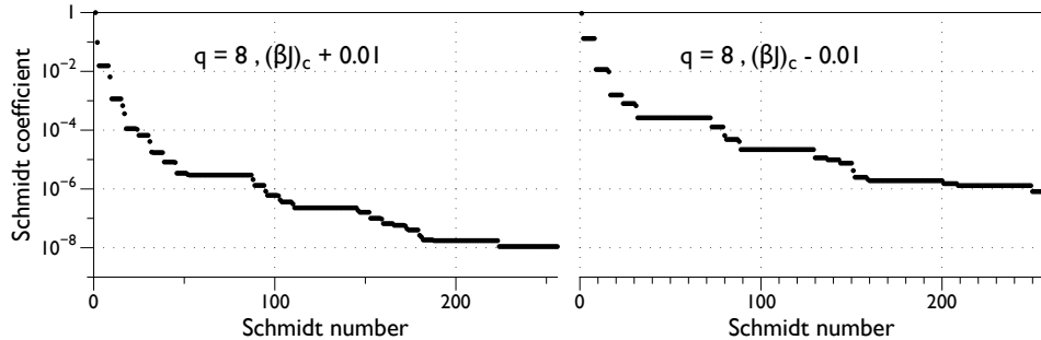
Figure 25: Spectrum of Schmidt coefficients (singular values) of the D = 256 MPS approximation to the fixed point of the transfer matrix of the q = 8 Potts model, in the ordered phase (left panel) and disordered phase (right panel). The smallest degeneracies appearing in the ordered (symmetry broken) phase are (q - 2) -fold, whereas in the disordered (symmetric) phase they are (q - 1) -fold.
