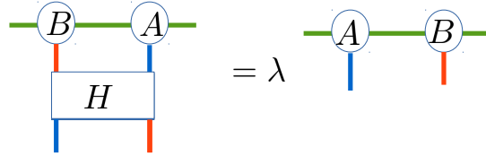
Figure 19: The zipper condition as a sufficient condition for having an exact eigenvector.
