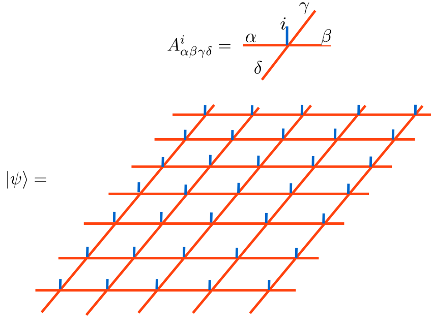
Figure 5: Definition of a projected entangled pair state parameterized by the tensor A_{\alpha\beta\gamma\delta}^i .
