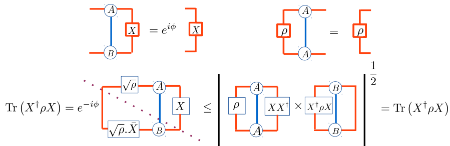
Figure 3: Graphical proof of the fundamental theorem of matrix product states.
