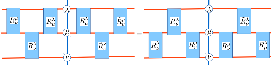
Figure 12: Yang-Baxter equations as associativity conditions for the R -matrices in the algebraic Bethe ansatz. We use the notation \tilde{R} for the inverse of R .
