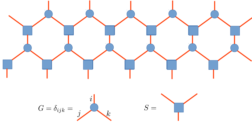
Figure 9: Matrix product operator representation of the cellular automaton for directed percolation.
