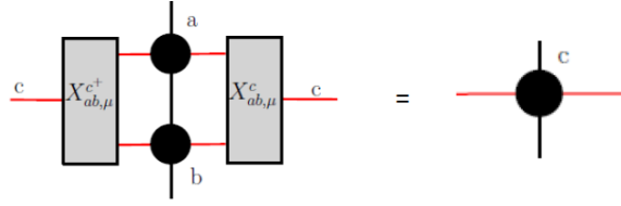
Figure 15: The fundamental theorem at work on a closed algebra of matrix product operators.
