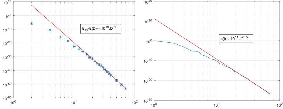
Figure 22: (a) Convergence of free energy versus bond dimension for the hard squares model and (b) decay of Schmidt coefficients for D = 70 .
