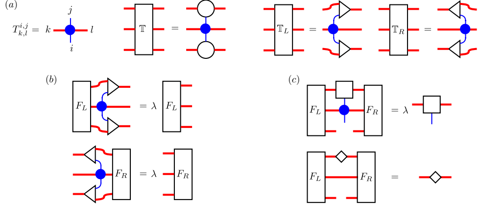
Figure 21: The MPO tensor and corresponding (transfer) matrices \mathbb{T} , \mathbb{T}_L and \mathbb{T}_R . At a stationary point for the MPS approximation of an MPO fixed point, the four eigenvalue problems in (b) and (c) are satisfied. The second eigenvalue problem in (c) follows from the first one in combination with the solutions of (b).
