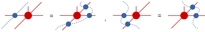
Figure 8: The local “pulling through” condition in topological projected entangled-pair states.
