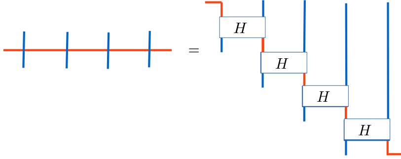
Figure 18: Rewriting a matrix product operator (MPO) in terms of a staircase. Note that the virtual dimension (red) in the staircase might be larger than the one in the original MPO.
