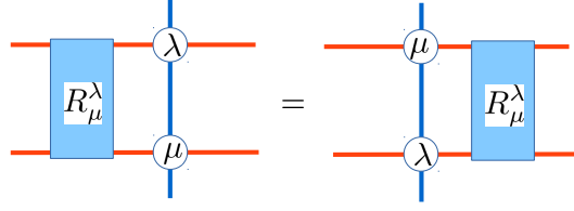
Figure 11: R -matrix as the gauge transformation switching O(\lambda) and O(\mu) .
