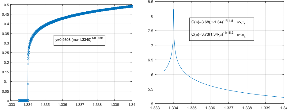
Figure 23: Magnetization and compressibility of the hard square model as a function of the chemical potential as calculated with the variational MPS method with bond dimension D = 128 .
